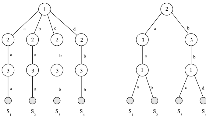
Figure 8.12: Two different tries for the same set of rule heads.
